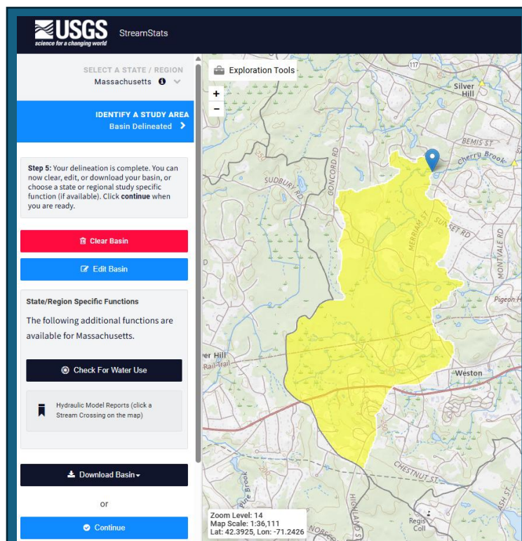
Figure 4: StreamStats Tool Example Watershed Delineation
